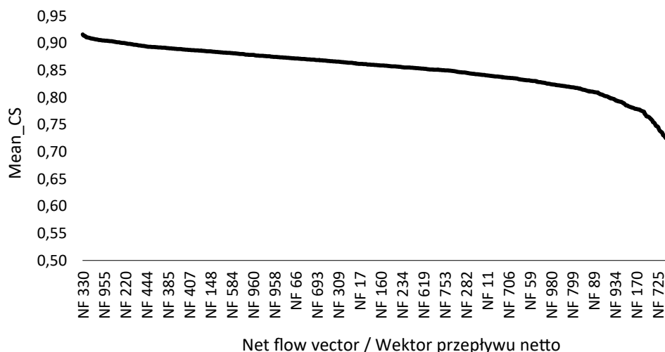
Figure 2. Values of the Mean_Cs function for the considered net flow vectors
